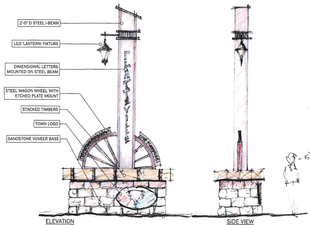
3 GATEWAY CONCEPT 3: I-BEAM & WHEEL SCALE: 1" = 2'-0" (±)
