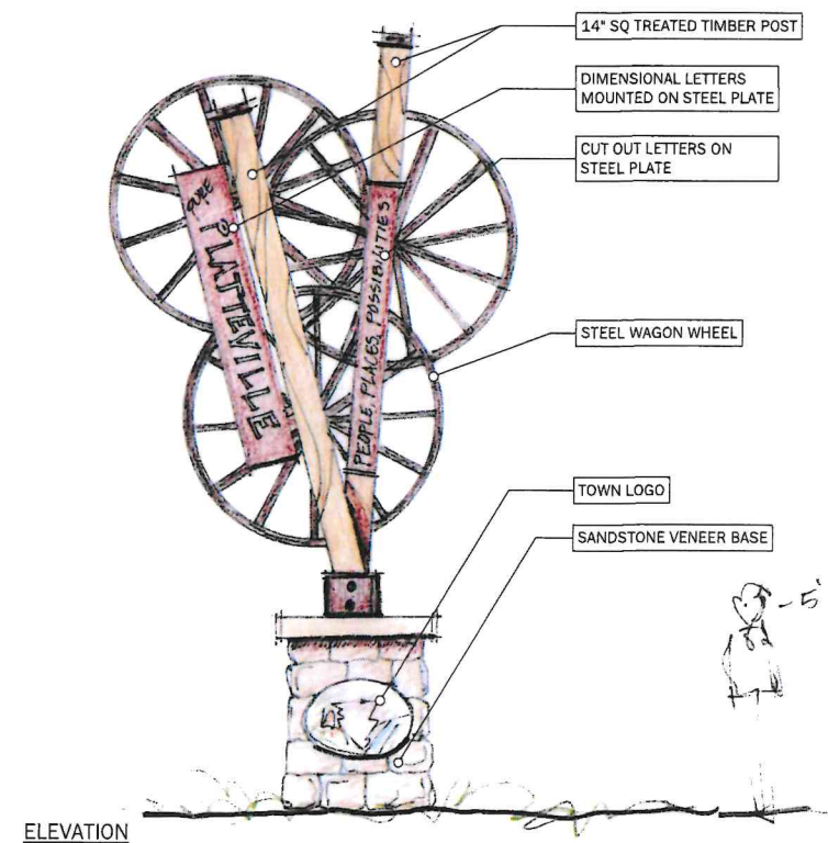
4 GATEWAY CONCEPT 4: TIMBER & WAGON WHEELS SCALE: 1" = 2'-0" (±)
